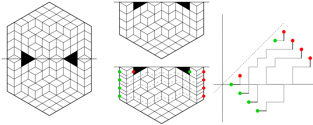
Fig. 3: Left: a horizontally symmetric tiling of H_{6,8} \setminus (\triangleright_4 \cup \triangleleft_4) . Middle (upper): the corresponding tiling of H_{6,8}^- \setminus (\triangleright_4 \cup \triangleleft_4) . Middle (lower): the corresponding set of lattice paths across dimers, where forced dimers are denoted by the thick black lines on the vertical sides. Right: the corresponding family of lattice paths in \mathbb{Z}^2 , here forced dimers correspond to forced east and north steps in black.
