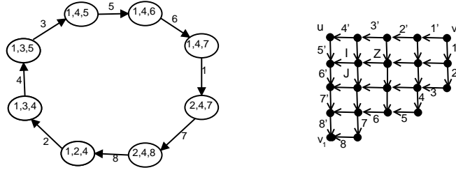
Fig. 5: The figure on the left is a circuit in G_{3,8} . The right figure is an oriented Young graph. Its inner boundary path formed by the edges labeled from 1' through 8'. Its outer boundary path formed by the edges labeled from 1 through 8, and all the vertices that appear along the latter path form the collection V .
