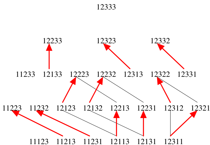
Fig. 2: The decomposition of the Stirling poset \Pi(5, 3) into Boolean algebras B_0, B_1 and B_2 . Based on the ranks of the minimal elements in each Boolean algebra, one can read the weight of the poset as S_q[5, 3] = 1 + 2(1 + q) + 3(1 + q)^2 + q^2 + 3q^2(1 + q) + q^4 .
