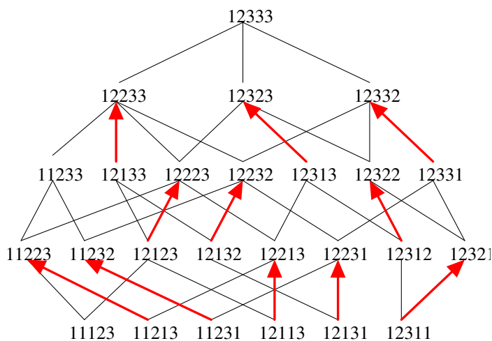
Fig. 1: The matching of the Stirling poset \Pi(5, 3) . The matched elements are indicated by arrows. The rank generating function for this poset is S_q[5, 3] = 6 + 8q + 7q^2 + 3q^3 + q^4 .
