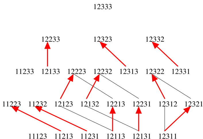
Fig. 2: The decomposition of the Stirling poset \Pi(5, 3) into Boolean algebras B_0 , B_1 and B_2 . Based on the ranks of the minimal elements in each Boolean algebra, one can read the weight of the poset as S_q[5, 3] = 1 + 2(1 + q) + 3(1 + q)^2 + q^2 + 3q^2(1 + q) + q^4 .
