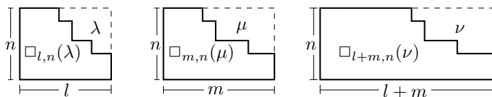
Fig. 2: The partitions occurring in the invariance relation of Theorem 1
