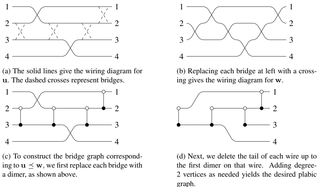
Fig. 3: Constructing a bridge graph from a bridge diagram. In this example, we have k = 2 , n = 4 , \mathbf{w} = s_1 s_2 s_3 s_2 s_1 s_2 , and \mathbf{u} = s_3 s_1 . Compare the figure at lower right with the bridge graph in Figure 1.
