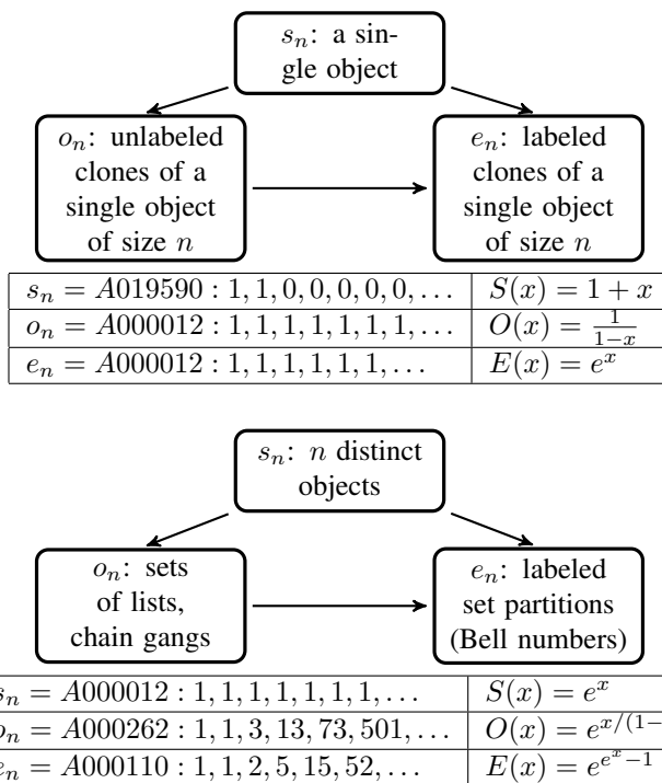
Fig. 6: Top: our garden has a single seed of a single vertex. Bottom: our garden has a single seed of n distinguishable objects. Strictly speaking, we are applying Theorem 4.1 to an extended category of posets that allow distinct “colors.”
