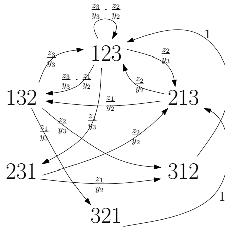
Fig. 2: Transition graph of the MSJMC with T = 3 and n_1 = n_2 = n_3 = 1 .
