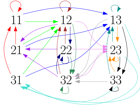
Fig. 3: The basic transition graph on St_2^3 . Note that the first letter has no effect on which states can be reached.
