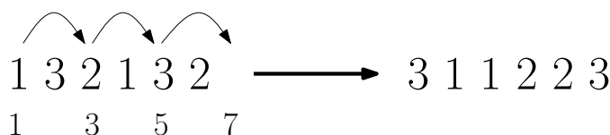
Fig. 1: A possible transition from the state 132132, corresponding to the bumping sequence (1, 3, 5, 7).
