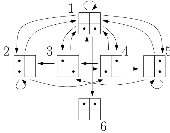
Fig. 4: The several jugglers Markov chain on the set space S_{2 \times 2, 2} .
