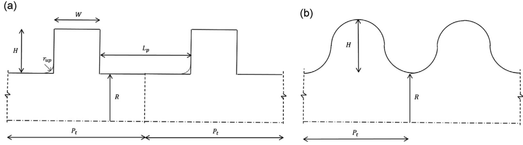
Fig. 3. Geometrical definitions for periodic pipes and channels: (a) refers to A1, B1, B2, C and D cases and (b) refers to the A2 and B3 cases.
