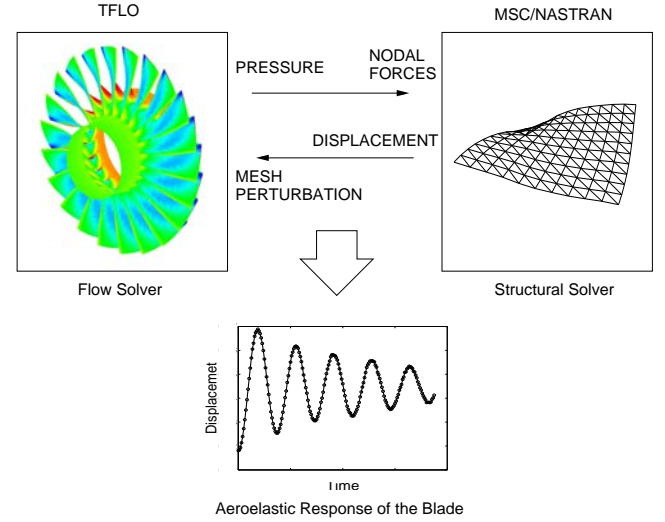
Figure 1. FLUID/STRUCTURE COUPLING
