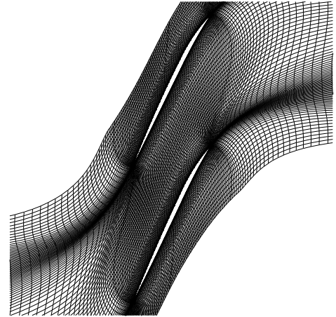
Figure 4. Blade-to-Blade View of Computational Grid for NASA Rotor 67
