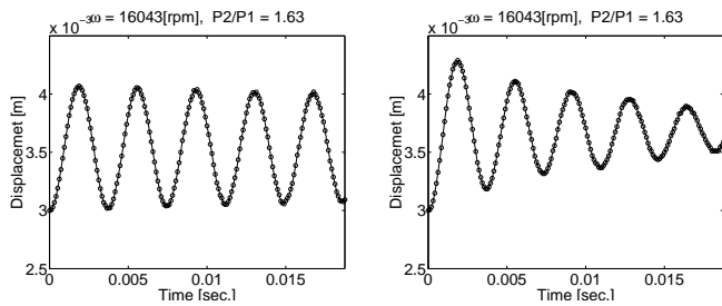
Figure 7. DEFLECTION AT MID-CHORD OF THE TIP SECTION FOR NEAR PEAK EFFICIENCY, \sigma = 0, 180 deg
