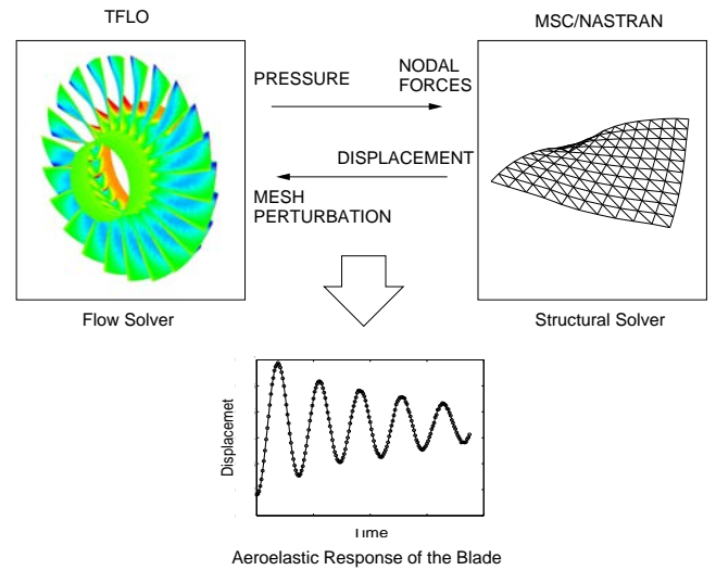
Figure 1. FLUID/STRUCTURE COUPLING
