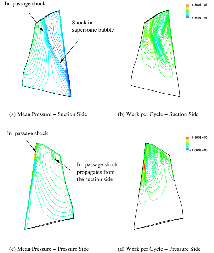
Figure 8. MEAN PRESSURE AND WORK PER CYCLE DISTRIBUTION ON THE BLADE SURFACES FOR NEAR PEAK EFFICIENCY, \sigma = 0 deg
