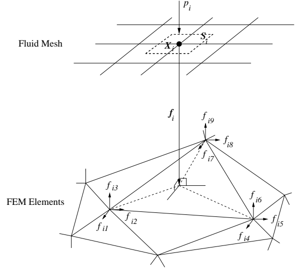
Figure 3. LOAD TRANSFER SYSTEM
