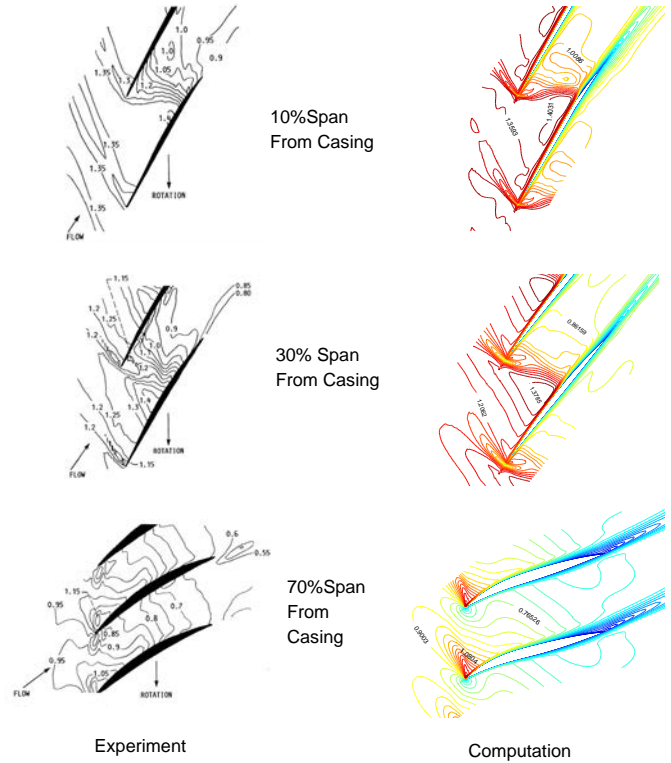
Figure 6. Experimental and Numerical Relative Mach Number Contour for Near Peak Efficiency
