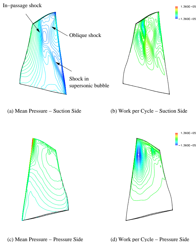
Figure 9. MEAN PRESSURE AND WORK PER CYCLE DISTRIBUTION ON THE BLADE SURFACES FOR NEAR PEAK EFFICIENCY, \sigma = 180^\circ
