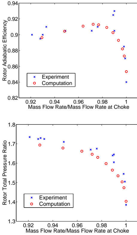
Figure 5. Comparison of Rotor Performance at Design Speed
