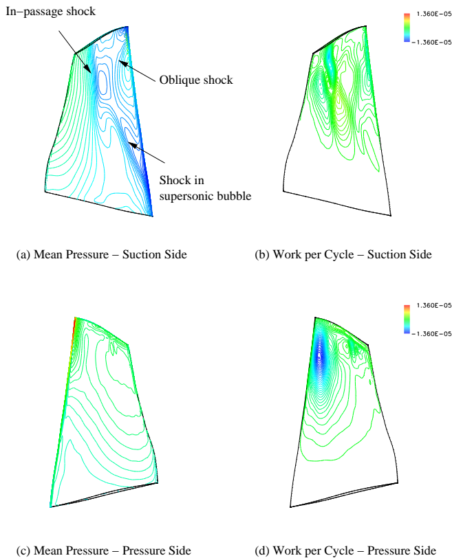
Figure 9. MEAN PRESSURE AND WORK PER CYCLE DISTRIBUTION ON THE BLADE SURFACES FOR NEAR PEAK EFFICIENCY, \sigma = 180\text{deg}
