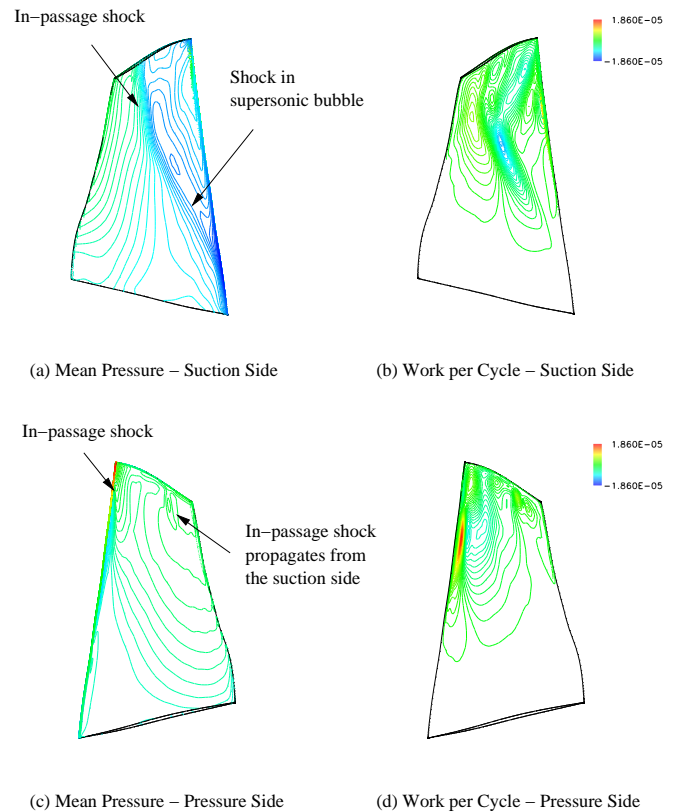
Figure 8. MEAN PRESSURE AND WORK PER CYCLE DISTRIBUTION ON THE BLADE SURFACES FOR NEAR PEAK EFFICIENCY, \sigma = 0 deg
