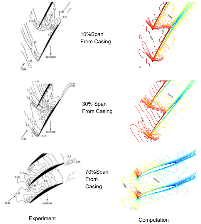
Figure 6. Experimental and Numerical Relative Mach Number Contour for Near Peak Efficiency
