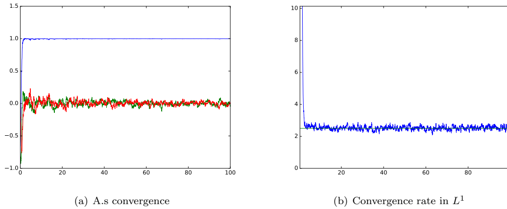
Figure 3: A.s. convergence of the three components of (\bar{\mu}_t)_t , \alpha = 2 , \Delta t = 2 \times 10^{-2} and \varepsilon_t = 0.1/(t+1)^{1/3} . The blue curve corresponds to the component of \bar{\mu}_t along b .
