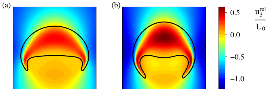
FIGURE 12. Influence of volume fraction on the deformation of an ordered array of dimpled ellipsoidal-cap bubbles (case C): vertical component of the relative velocity ( \mathbf{u}^{\text{rel}} = \mathbf{u} - \langle \mathbf{u} \rangle_d ) in a vertical symmetry plane passing through the center of a bubble. Increasing volume fractions from left to right: (a) \phi = 0.2\% , U/U_0 = 1.22 , and (b) \phi = 2.4\% , U/U_0 = 1.17 . Same conventions as in figure 11. Only the region near and inside a bubble is shown.
