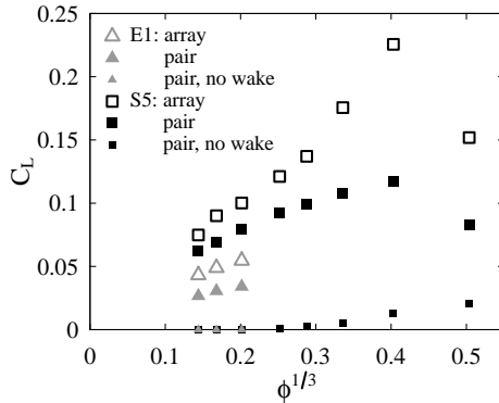
FIGURE 16. Average lift coefficient as a function of volume fraction for case E1 (grey triangles) and case S5 (black squares). Open symbols: for a bubble of an ordered array, present DNS. Filled symbols: for the trailing bubble of a pair of spherical bubbles within the same conditions (orientation, Reynolds number, separation distance) as two vertically-aligned bubbles of the ordered array, with (large symbols) and without (small symbols) accounting for the interaction with the wake of the leading bubble, from Hallez & Legendre (2011).
