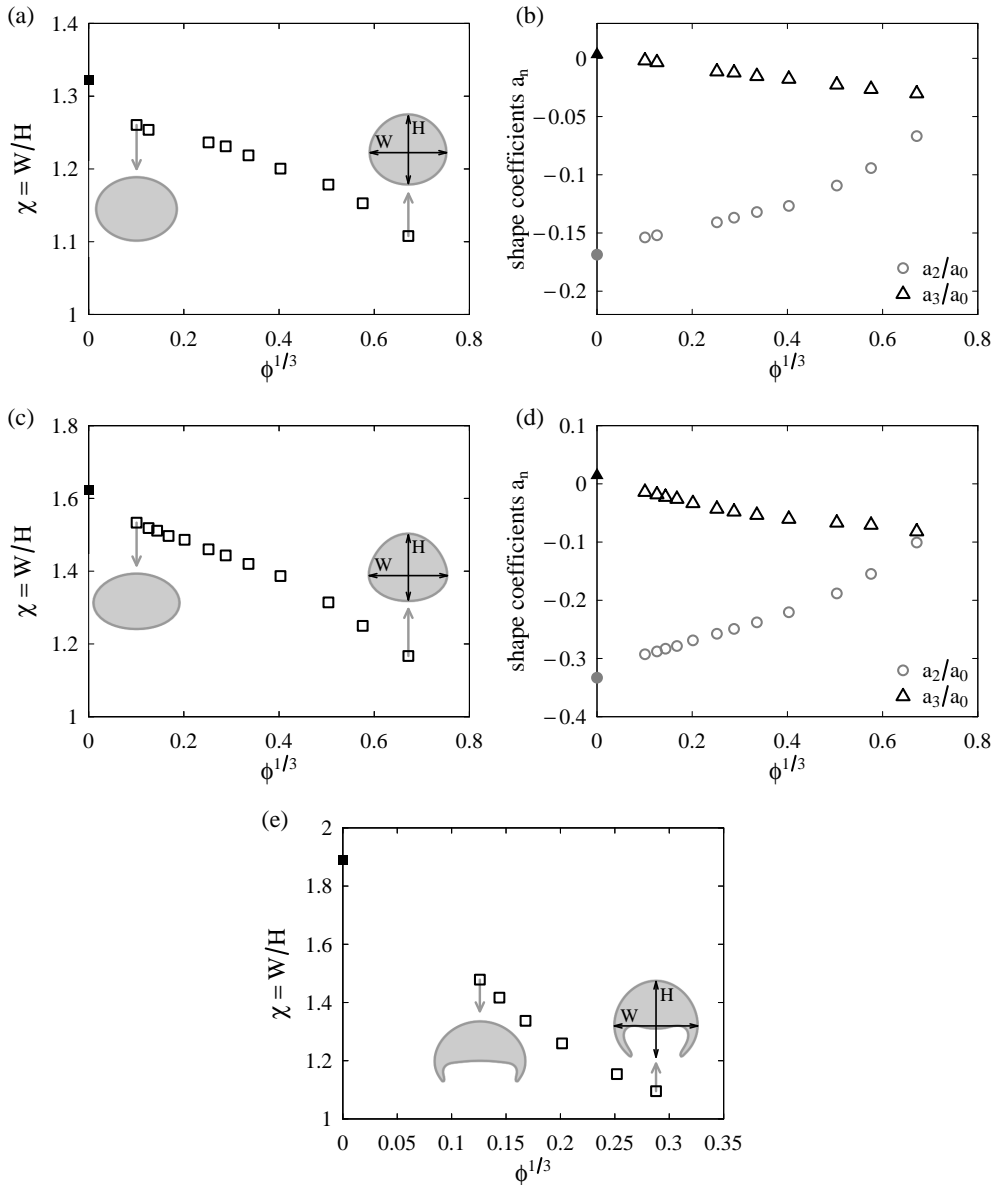
FIGURE 10. Steady aspect ratio (a,c,e) and shape coefficients (b,d) of bubbles in an ordered array configuration as a function of volume fraction for: (a,b) case E1 ( Bo = 2.0 , Ar = 29.9 ); (c,d) case E2 ( Bo = 5.0 , Ar = 30.0 ); (e) case C ( Bo = 243 , Ar = 15.2 ). Bubbles shapes are shown in grey for the highest and the lowest simulated volume fractions. Open symbols: DNS. Filled symbol: isolated bubble (aspect ratios estimated from Loth (2008) for cases E1 and E2 and from Hua et al. (2008) for case C; shape coefficients estimated from Ryskin & Leal (1984)).
