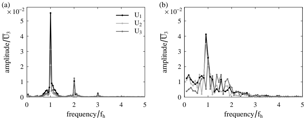
FIGURE 18. Single-sided amplitude spectra of discrete Fourier transforms of the drift velocity components time signals. Unsteady oblique rise of ordered arrays of bubbles: (a) oscillatory motion (case S5 at \phi = 3.8\% ), (b) chaotic motion (case S5 at \phi = 1.6\% ). The amplitude is normalized by the average vertical drift velocity \overline{U}_3 , the frequency is normalized by f_h = (\overline{U}_1 + \overline{U}_2)/(2h) .
