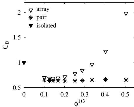
FIGURE 7. Drag coefficient as a function of volume fraction for case S4. \nabla : ordered array; * : trailing bubble of a vertically-aligned pair within the same conditions (Reynolds number, separation distance), from Hallez & Legendre (2011); \blacktriangledown : isolated bubble, estimated from Mei et al. (1994).
