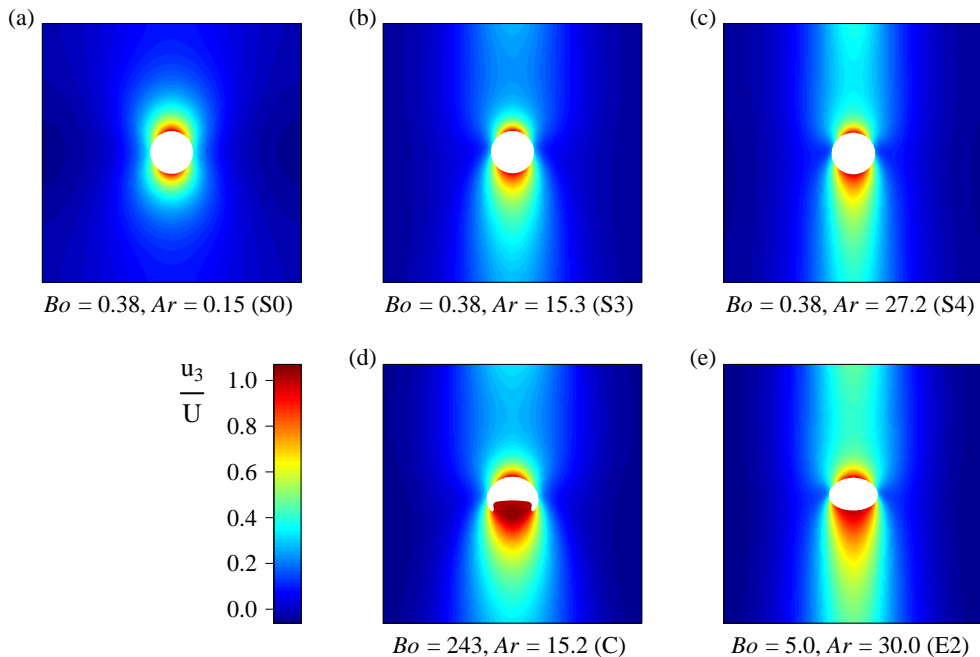
FIGURE 5. Vertical component of the liquid velocity normalized by the bubble drift velocity in a vertical symmetry plane passing through the center of a bubble in an ordered array configuration at \phi = 0.2\% . Gravity is pointing downward ( \mathbf{g} = -ge_3 ). Increasing Archimedes numbers from left to right, and increasing Bond numbers from top to bottom.
