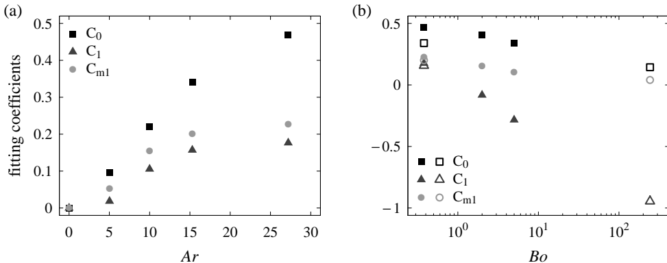
FIGURE 9. Fitted coefficients for U(\phi)/U_0 as given by (4.8): (a) as a function of the Archimedes number for Bo = 0.38 , (b) as a function of the Bond number for Ar \approx 15 (open symbols) and for Ar \approx 30 (filled symbols). The coefficients are obtained by least-squares fits of DNS and isolated-bubble data.
