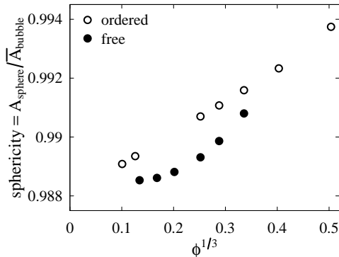
FIGURE 22. Influence of volume fraction on the bubbles sphericity in ordered (open circles) and free (filled circles) arrays for case E1. The sphericity is defined as the ratio between the total surface areas of a set of N_b volume-equivalent spheres and that of the bubbles.
