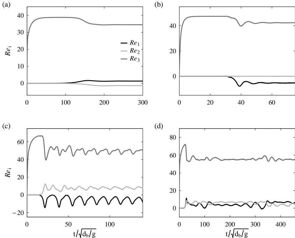
FIGURE 14. Time signals of the bubble drift velocity components (given as Reynolds numbers Re_i = \rho_c U_i d_b / \mu_c ), with \mathbf{U} = U_i \mathbf{e}_i and gravity pointing in the -\mathbf{e}_3 direction, in the three regimes of motion: steady oblique rise (a,b), oscillatory oblique rise (c), and chaotic oblique rise (d). These regimes are obtained for (a) case E1 at \phi = 0.8\% , (b) case S5 at \phi = 13\% , (c) case S5 at \phi = 3.8\% , (d) case S5 at \phi = 0.5\% .
