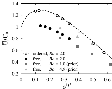
FIGURE 21. Influence of volume fraction on the bubbles drift velocity in ordered and freely evolving suspensions, with comparable Ar ( \approx 30 ) and various Bo . The drift velocity is normalized by the terminal velocity of an isolated bubble for the same Archimedes and Bond numbers (estimated from Loth (2008)). \circ and --- : present DNS data, and their numerical fit, for N_b = 1 (ordered arrays) and Bo = 2.0 ; \bullet : present DNS for free arrays of 8 bubbles with Bo = 2.0 ; \blacksquare : prior DNS of Bunner & Tryggvason (2002a) for free arrays of 27 bubbles with Bo = 0.98 ; \blacktriangle : prior DNS of Bunner & Tryggvason (2003) for free arrays of 27 bubbles with Bo = 4.9 .
