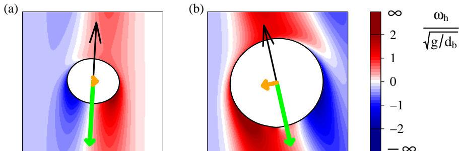
FIGURE 17. Liquid vorticity horizontal component \omega_h = \boldsymbol{\omega} \cdot \mathbf{e}_h in the vertical plane passing through the center of a bubble and containing its drift velocity, for ordered arrays of bubbles rising steadily in an oblique direction: (a) case E1, \phi = 0.8\% ; (b) case S5, \phi = 6.5\% . Positive (negative) values upstream of the bubble would give a positive (negative) contribution to the lift force as modeled by (4.12). The thin black arrow shows the direction of bubble drift velocity. The thick arrows show the magnitudes and directions of the drag (green arrows) and lift (orange arrows) forces scaled by the buoyancy force.
