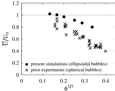
FIGURE 23. Influence of volume fraction on the normalized drift velocity of freely rising bubbles: comparison between simulations and experiments. ●: present DNS ( N_b = 8 , Ar = 29.9 , Bo = 2.0 , Re_0 = 31 ); ×: experiments of Martinez-Mercado et al. (2007) ( Ar = 26.3 \pm 1.6 , Bo = 0.25 \pm 0.02 , Re_0 = 29.7 \pm 3.1 ). The terminal velocities U_0 in unbounded liquid have been estimated from the correlation of Loth (2008) for numerical simulations (ellipsoidal bubbles) and from the correlation of Mei et al. (1994) for experiments (spherical bubbles).
