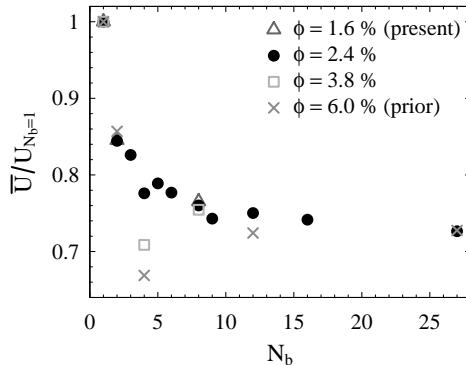
FIGURE 19. Influence of the number of bubbles on the average bubbles drift velocity for various volume fractions. The drift velocity is normalized by that obtained in the ordered configuration ( N_b = 1 ). Symbols other than crosses: present DNS for case E1 ( Ar = 29.9 , Bo = 2.0 ). Crosses: prior DNS of Bunner & Tryggvason (2002a) for a comparable flow regime ( Ar = 29.7 , Bo = 0.98 ).
