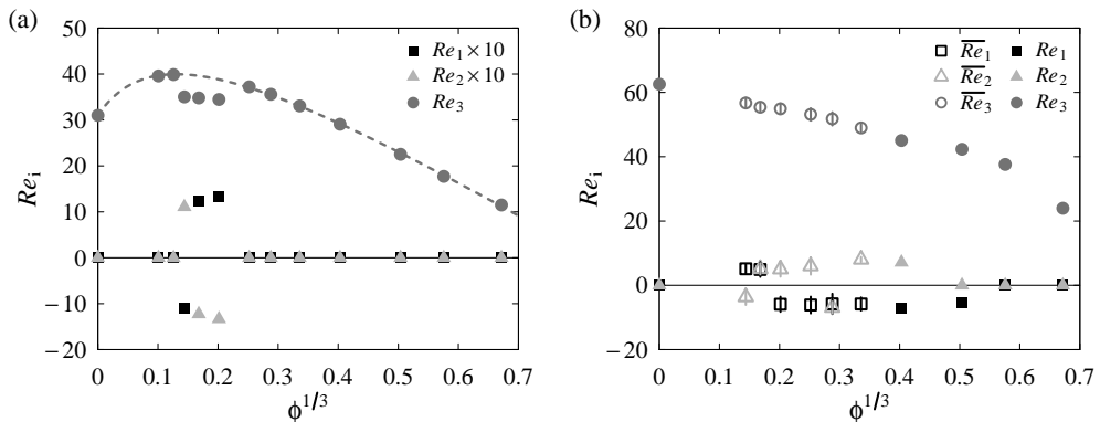
FIGURE 15. Quasi-steady drift velocity components ( \mathbf{U} = U_i \mathbf{e}_i ) in the form of Reynolds numbers ( Re_i = \rho_c U_i d_b / \mu_c ) as a function of volume fraction for an ordered array of bubbles in the cases where bubbles exhibit non-vertical motions. Gravity is pointing in the -\mathbf{e}_3 direction. (a) Case E1 ( Bo = 2.0 , Ar = 29.9 , note that the horizontal components have been multiplied by 10 for clarity). (b) Case S5 ( Bo = 0.38 , Ar = 40.7 ). Filled symbols are used when the bubbles motion is steady (oblique or vertical). Open symbols and vertical bars are used when the bubbles motion is unsteady: symbols indicate the mean drift velocity, and bars show its root mean square. The dashed line is a numerical fit of the form of (4.8) matching DNS and isolated-bubble data for the vertical rise only.
