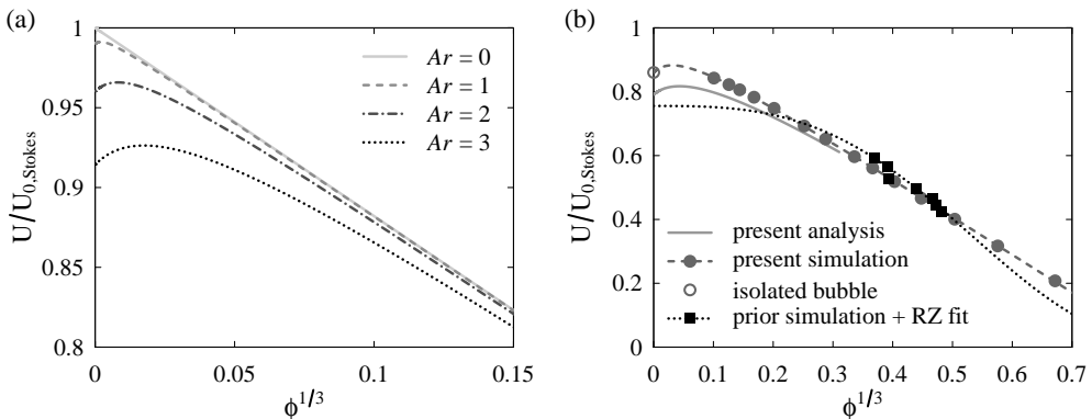
FIGURE 3. Steady drift velocity of an ordered array of spherical bubbles, normalized by the terminal velocity of an isolated bubble in Stokes flow conditions, as a function of volume fraction for small Archimedes numbers. (a) The effect of small but finite Ar , from Oseen-flow analysis. (b) Comparison of analytical and numerical solutions for Ar = 5.03 (case S1). Analytical solutions are obtained from (4.3). In (b), —: analysis; ●: DNS; ○: isolated bubble, estimated from Mei et al. (1994); - - -: numerical fit of the form of (4.8) matching DNS and isolated-bubble data; ■ and ·····: numerical data and fit by a Richardson-Zaki relation from Sankaranarayanan et al. (2002).
