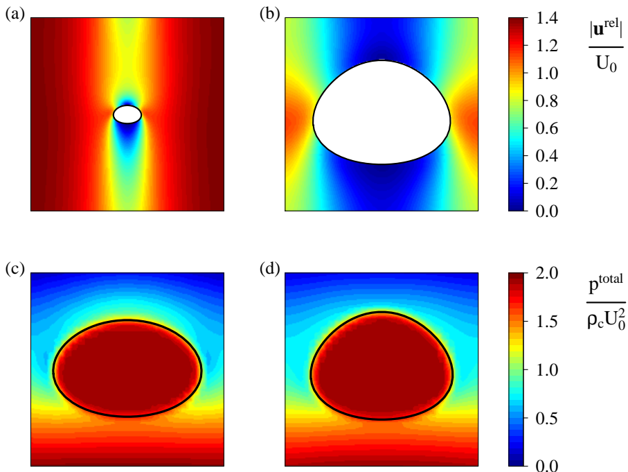
FIGURE 11. Influence of volume fraction on the deformation of an ordered array of oblate ellipsoidal bubbles (case E2): relative velocity ( \mathbf{u}^{\text{rel}} = \mathbf{u} - \langle \mathbf{u} \rangle_d ) and pressure fields in a vertical symmetry plane passing through the center of a bubble. Increasing volume fractions from left to right: (a,c) \phi = 0.1\% , U/U_0 = 1.34 , and (b,d) \phi = 13\% , U/U_0 = 0.73 . Top row: magnitude of the liquid relative velocity in the entire unit cell. Bottom row: total pressure (including the mixture-average hydrostatic component) near and inside a bubble. Gravity is pointing downward ( \mathbf{g} = -g\mathbf{e}_3 ). The black lines show the interface location.
