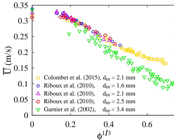
FIGURE 24. Prior experimental data for air bubbles rising in water: \bar{U} (average drift velocity in meters per second) replotted versus \phi^{1/3} (with \phi the gas volume fraction). In the legend, d_{b0} is the experimentally-determined bubble diameter at zero volume fraction.
