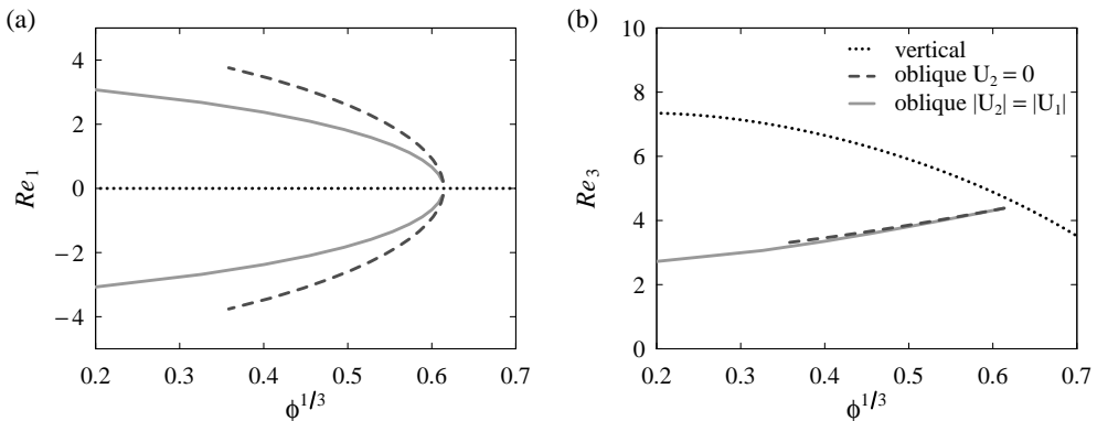
FIGURE 13. Subset of analytical solutions obtained from solving (B3) for Ar = 20 and \rho_d/\rho_c = \mu_d/\mu_c = 0 : bubble drift velocity horizontal (a) and vertical (b) components, given as Reynolds numbers Re_i = U_i \rho_c d_b / \mu_c , as a function of volume fraction. Gravity is pointing in the -\mathbf{e}_3 direction. \cdots\cdots : vertical rise ( U_1 = U_2 = 0 ); --- : oblique rise with U_2 = 0 ; --- : oblique rise with |U_2| = |U_1| .
