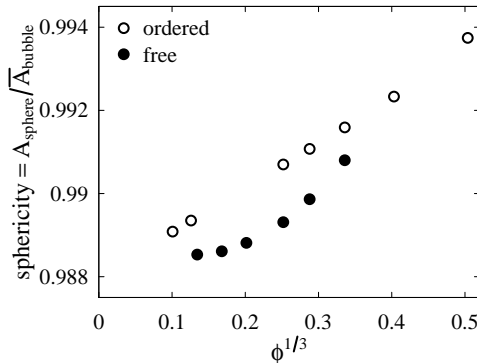
FIGURE 22. Influence of volume fraction on the bubbles sphericity in ordered (open circles) and free (filled circles) arrays for case E1. The sphericity is defined as the ratio between the total surface areas of a set of N_b volume-equivalent spheres and that of the bubbles.
