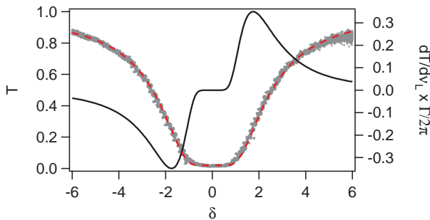
FIG. 2: Grey curve: experimental probe transmission as a function of the laser detuning. Red (dashed) curve: fit of the transmission curve, giving an on-resonant optical thickness of 19. Black curve: fit derivative used for the intensity to frequency noise conversion (right axis).
