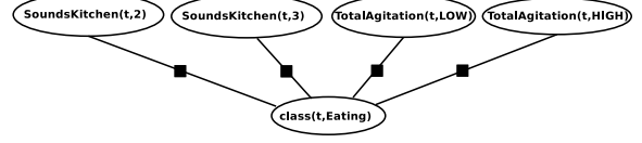
Fig. 4. Ground Naive MLN.
