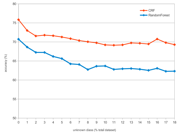
Fig. 7. Accuracy against percentage of windows belonging to the Unknown class for Random Forest and CRF applied to the HIS database.
