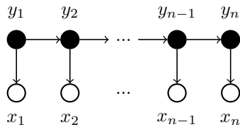
Fig. 2. Representation of a classical HMM for labelling elements in a sequence: y_i are the hidden states, x_i are the observations
