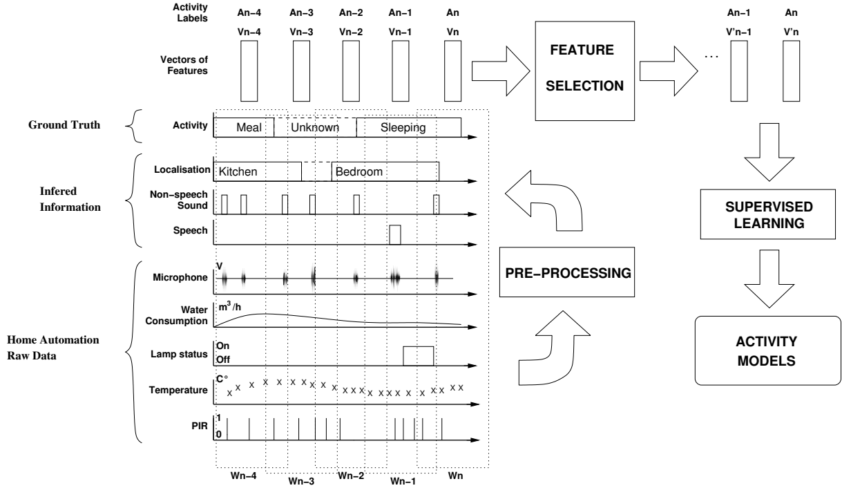
Fig. 1. Diagram of the overall methodology for activity model determination.
