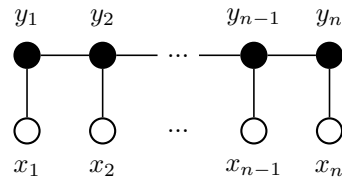
Fig. 3. Representation of a CRF for labelling elements in a sequence
