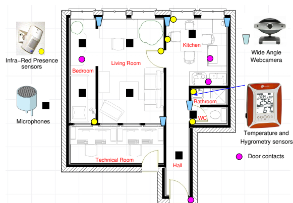
Fig. 6. Equipment and layout of the Health Smart Home (HIS) of the TIMC-IMAG Laboratory in Grenoble
