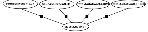
Fig. 4. Ground Naive MLN.
