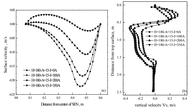
Fig. 4: Surface velocity at steel/slag interface and vertical velocity V_y near narrow face of mold
