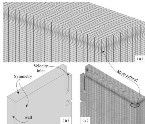
Fig. 1: Schematics of geometrical model (a) Refined mesh; (b) Fluid zone; (c) Hexahedral structured mesh of fluid zone
