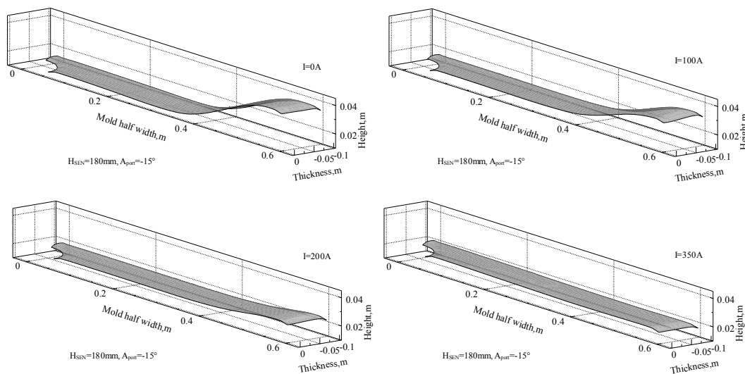
Fig. 3: Steel/slag interface profiles with different current density
