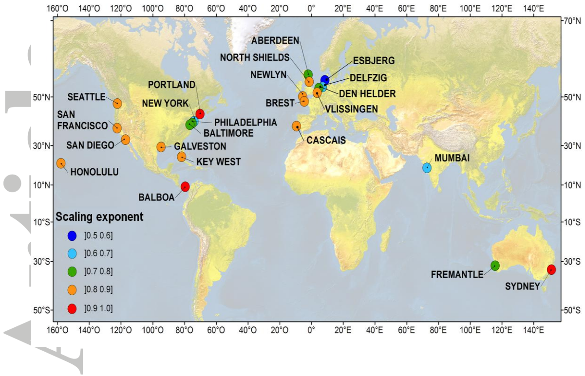
Fig. 2. Location of the 23 historic tidal records and magnitude of the observed scaling exponent.
