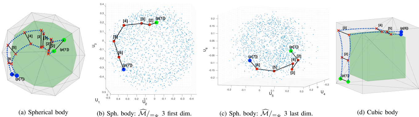
Fig. 8. Motion planning, performed with the agent endowed with two fingertips, and for a spherical or cubic body. The two trajectories on the actual agent body are shown in (a) and (d) for the two body geometries. The corresponding path in the discrete motor quotient set \widehat{\mathcal{M}}/\equiv_{\psi} , where the interpolation is actually performed, is shown in (b) and (c) for the spherical body. The same color conventions as in Figure 7 are used.
