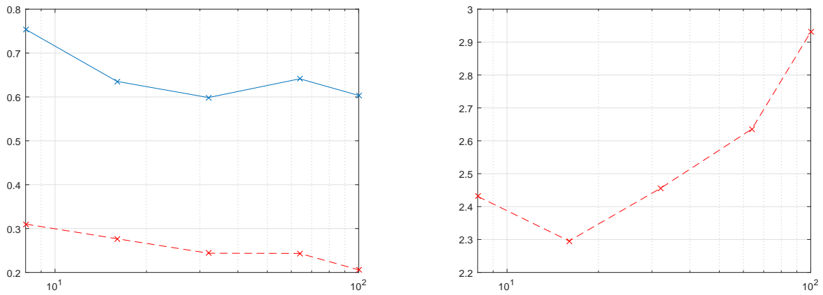
Figure 4: Recovery on a box: risk bounds as functions of problem dimension n , noise level \sigma = 0.01 . Left plot: upper bound of the risk of linear recovery (solid blue line) and lower bound on \text{Risk}_{\text{opt}} (red dash line). Right plot: suboptimality ratio.
