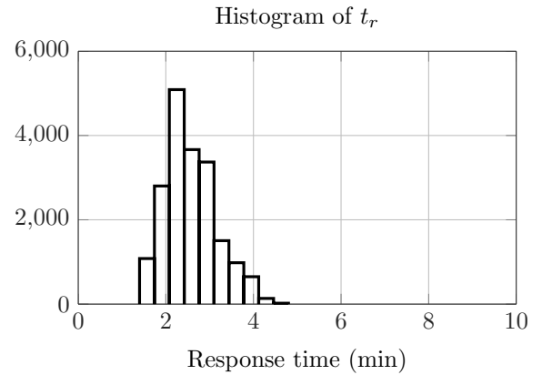
Fig. 2. Histogram of the response times for the 19299 sampled patients used in the computation of the probabilistically certified response time.
