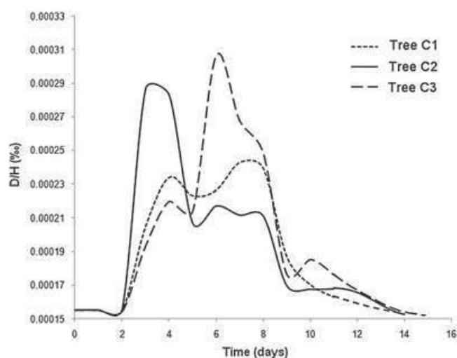
Figure 3. Time course of D atom % values of water extracted from the leaf canopy for Ceriops trees.
