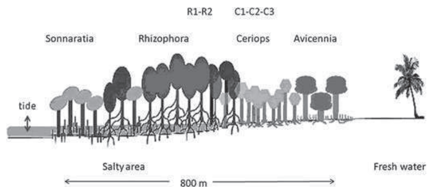
Figure 2. Zonation of the mangrove of Malamani (modified from Herteman [34] ) and location of the sampled trees: R1 and R2 for Rhizophora strata and C1–C3 for the Ceriops strata .
