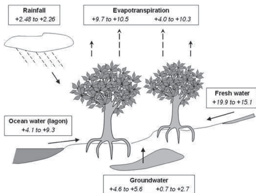
Figure 5. Synoptic figure of the water circulation and the \delta D values of the different water pools, in relation the obtained evaporated water before the D 2 O injection.
