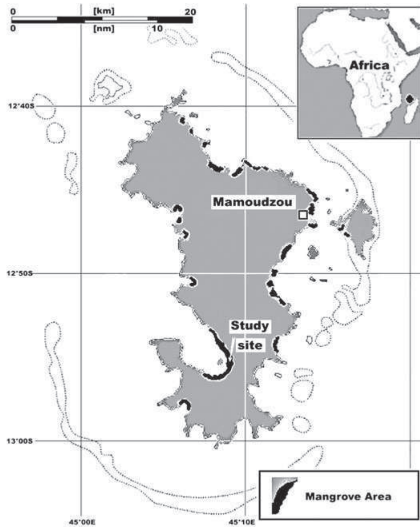
Figure 1. Location of the mangrove forest (black) and the study site in the Chirongui Bay on Mayotte, Comores Islands, Indian Ocean.
