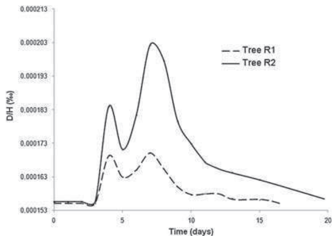
Figure 4. Time course of D atom % values of water extracted from the leaf canopy for Rhizophora trees.
