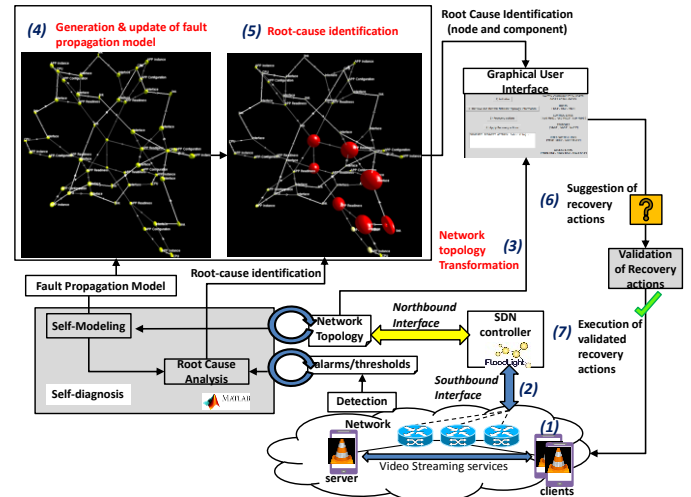
Figure 2. Demo Scenario of the THESARD platform
