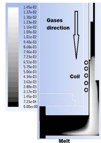
Fig. 7: Mole Fraction of O radicals (experiment 5)
