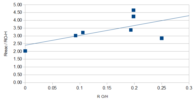
Fig. 4: Link between R_{react}/R_{O-H} and R_{O/H}
