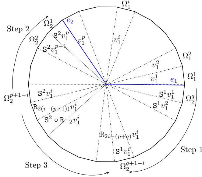
Figure 11: Scheme representing steps 1)-2)-3) for building R_i^{\text{adm}} .
