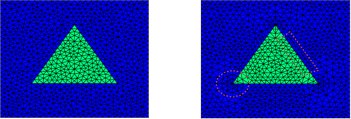
Figure 8: (Left) example a standard triangulation of \Omega_h (1430 nodes); (right) example of locally T-conforming mesh (1424 nodes). The dashed lines enclose regions where we built T-conforming meshes near a corner, respectively a straight line.
