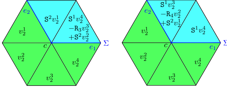
Figure 4: Representation of the two admissible geometry-based operators \mathbf{R}'^{\text{adm}} : (left) one applies an axial symmetry in \Omega_2^1 to reach \Omega_1^1 and folds the rest of v_2 into \Omega_1^1 to ensure continuity; (right) one applies an axial symmetry in \Omega_2^4 to reach \Omega_1^1 and folds the rest of v_2 into \Omega_1^2 to ensure continuity.
