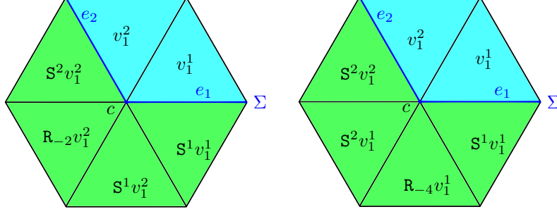
Figure 3: Representation of the two admissible geometry-based operators \mathbf{R} .
