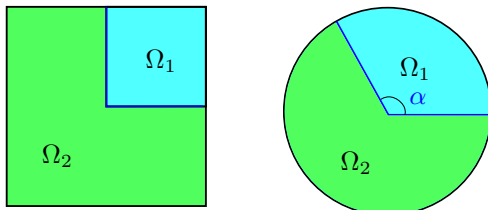
Figure 1: Examples of geometries that have been handled with the T-coercivity: (left) a square where \Omega_1 is one quadrant; (right) a disk where \Omega_1 is an angular sector of angle \alpha .
