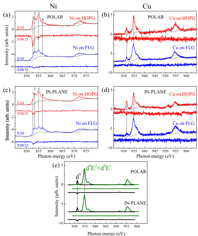
FIG. 4: XAS and XMCD spectra of Ni and Cu adatoms after substrate background subtraction measured at T = 8\text{K} and B = 5\text{T} for polar (a-b) and in-plane (c-d) geometries. Respective coverages are 0.017ML for Ni and 0.005ML Cu atoms on HOPG, as well as 0.023ML Ni and 0.005ML Cu on FLG. Simulated XAS and XMCD spectra are shown in (e) for an incoherent superposition of Cu d^9 with crystal field ( D_{3q} = 1\text{eV} , D_\sigma = -0.04\text{eV} , D_\tau = -0.02\text{eV} ) and Cu d^8E^2 + d^9E^1 with crystal field ( D_{3q} = 2\text{eV} , D_\sigma = 0.14\text{eV} , D_\tau = 0.08\text{eV} ).
