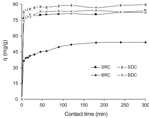
Fig. 6. Kinetics of the adsorption of MG by the clays: C_0=100 mg/L, R=1 g/L, pH=7.5 , T=25 °C, Agitation=500 rpm.
