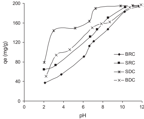
Fig. 3. Effect of pH on the adsorption of MG by the clays: C_0=100 mg/L, R=0.5 g/L, contact time=120 min, T=25 °C, Agitation=500 rpm.
