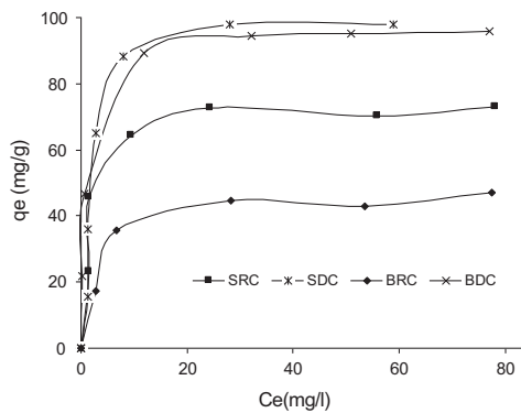
Fig. 8. Effect of MB concentration on its adsorption by the clays: V=200 mL, R=1 g/L, \text{pH}=7.5 , T=25 °C, Agitation=500 rpm.
