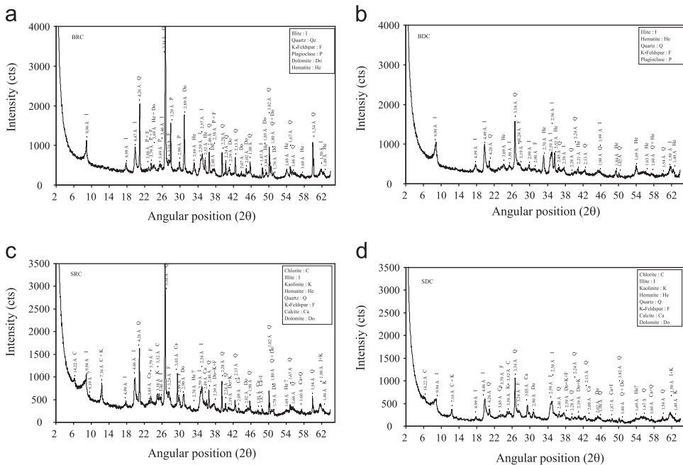
Fig. 1. (a) XRD patterns of Berrechid raw clay (BRC). (b) XRD patterns of Berrechid decanted clay (BDC). (c) XRD patterns of Safi raw clay (SRC). (d) XRD patterns of Safi decanted clay (SDC).
