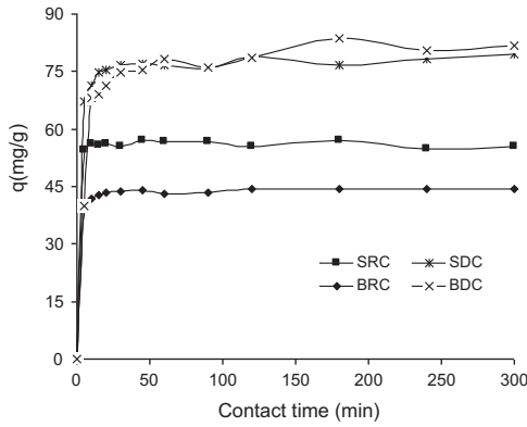
Fig. 5. Kinetics of the adsorption of MB by the clays: C_0=100 mg/L, R=1 g/L, pH=7.5 , T=25 °C, Agitation=500 rpm.
