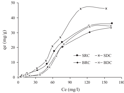
Fig. 10. Effect of MO concentration on its adsorption by the clays: V=200 mL, R=1 g/L, pH=6.5 , T=25 °C, Agitation=500 rpm.
