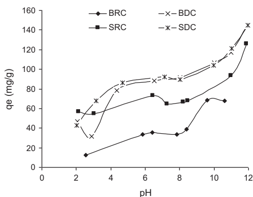
Fig. 2. Effect of pH on the adsorption of MB by the clays: C_0=100 mg/L, R=0.5 g/L, contact time=120 min, T=25 °C, Agitation=500 rpm.
