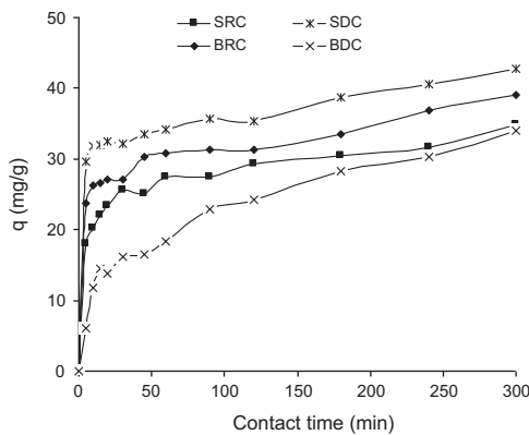
Fig. 7. Kinetics of the adsorption of MO by the clays: C_0=100 mg/L, R=2 g/L, pH=6.5 , T=25 °C, Agitation=500 rpm.
