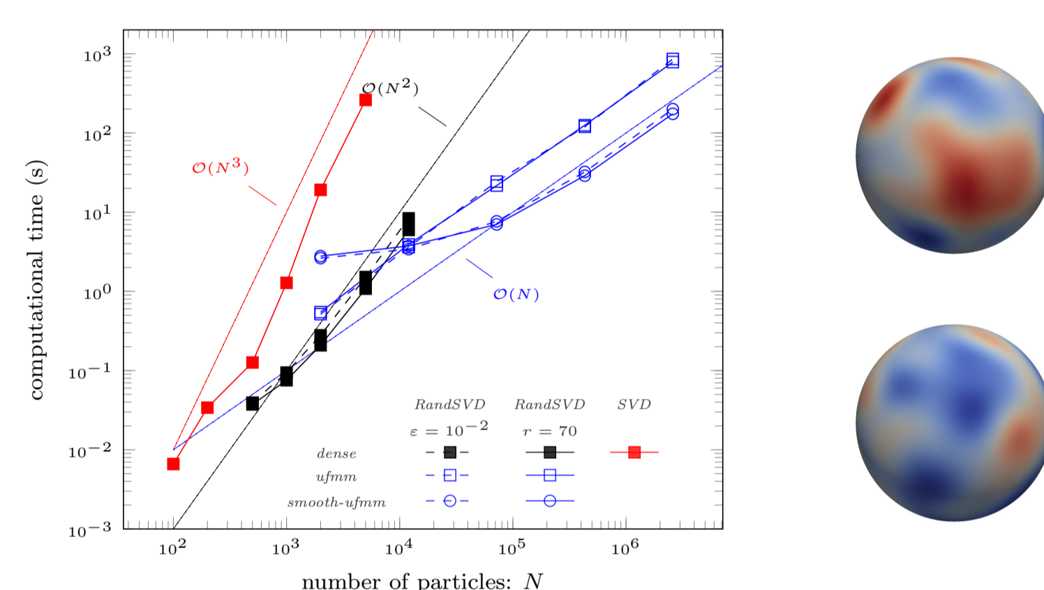
FIGURE 2: Left: Running time for computing a randomized SVD using either the fixed rank or fixed accuracy algorithm with q = 0 and s = 10 . Matrices are multiplied either in a dense way (filled black squares) or by means of a fmm scheme, particles are randomly distributed on the unit sphere and the correlation is Gaussian ( k_{\infty} ) with \ell = 0.5 . Right: Realizations on the unit sphere with 72k points, k_{\infty} and \ell = 0.25 using FMM accelerated SVD (top) and smooth variant (bottom).
