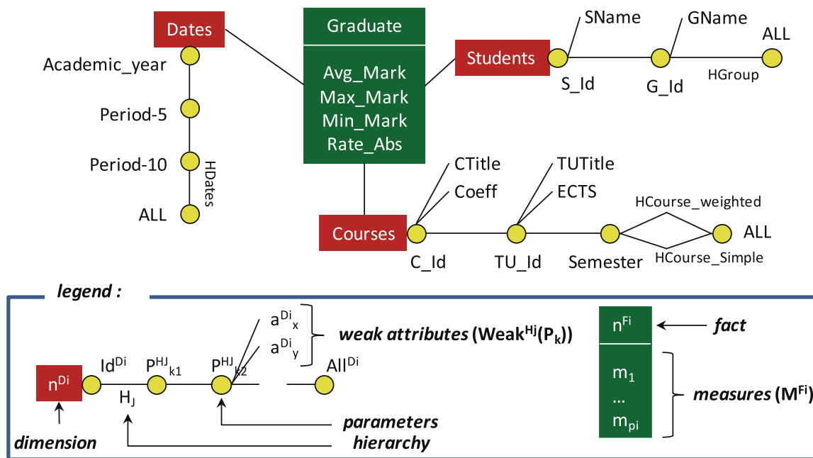
Fig. 2. The MDB of the diploma delivery case study
