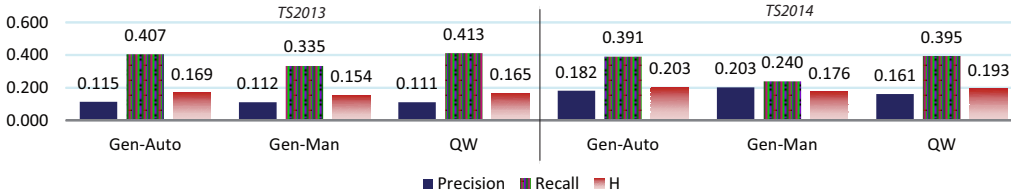
Fig. 1: Comparison of the different strategies for trigger term selection (Gen-Auto, Gen-Man, QW)
