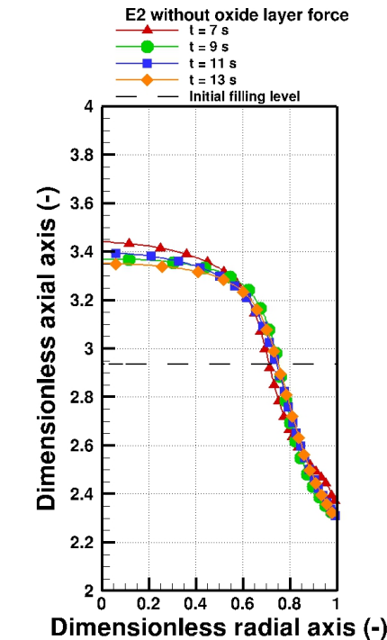
Fig. 6: Temporal evolution of dome profiles – E2.
