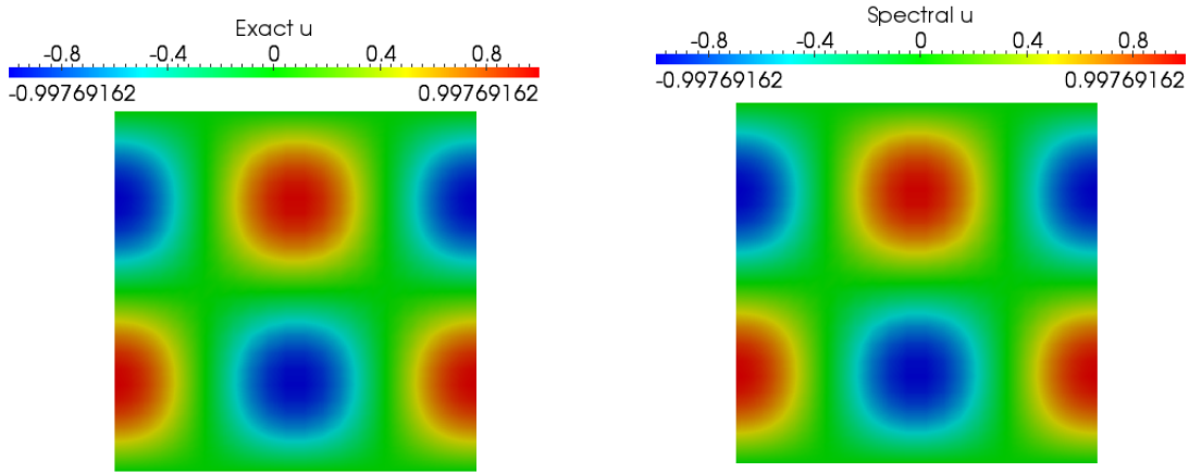
Figure 3: Isovalues of the the exact solution (7.1) at the final time (left) and of the spectral
