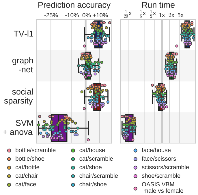
Fig. 1. Prediction accuracy and computation time for different classification tasks from brain images: 14 on the Haxby dataset, and gender prediction on OASIS. Values are displayed relative to the mean over 4 classifiers: TV- \ell_1 , graph-net, social sparsity, and a linear SVM with 20% univariate feature selection. Each subject of the Haxby study gives one data point.
