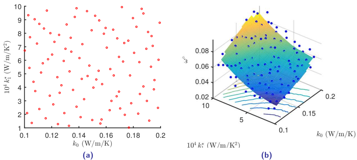
Figure 7. Halton quasi-random sampling of parameters (k_0, k_1) (a) and frequency optimal experiment design \omega^o (b).
