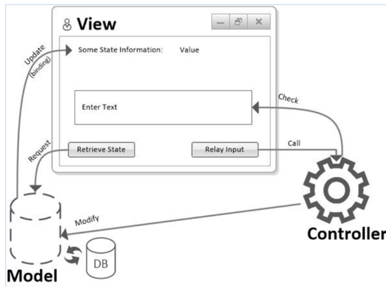
Figure 1: The Model-View-Controller [9]
