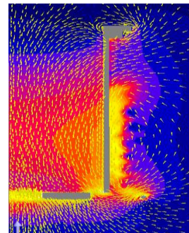
Fig. 3. Validation example of induction simulation of an empty cold crucible. The Joule losses in the parts of the crucible are compared for the same inductor current. On the left, magnetic field in a vertical cross plane of the cold crucible.
