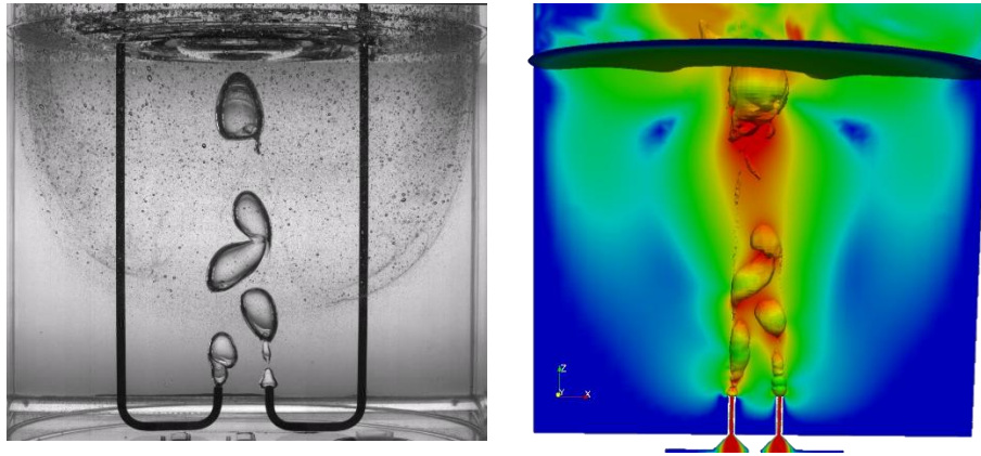
Fig. 4. Diphasic simulation of the interaction of two bubble columns in a viscous fluid representative of molten glass. Left, experimental view of oil, right CFD with Openfoam.
