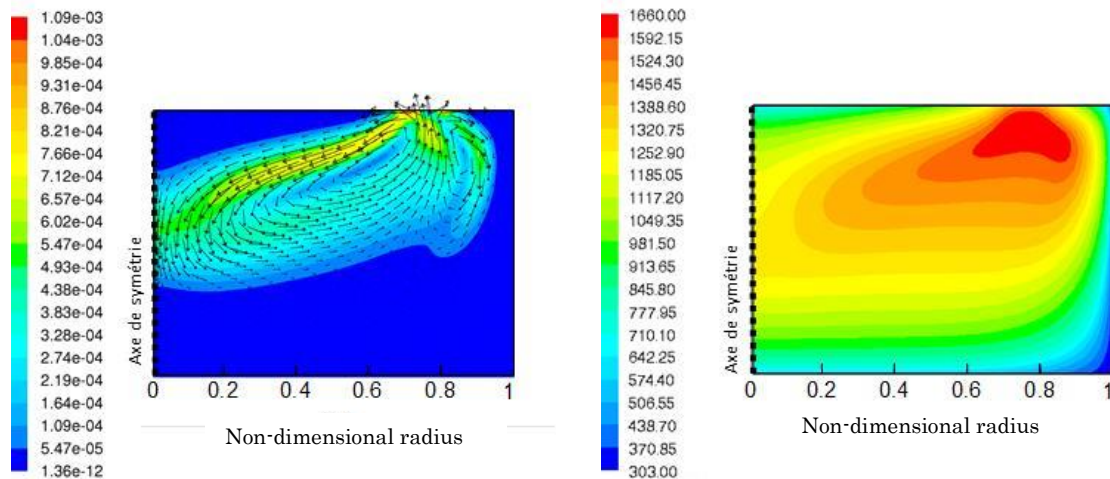
Fig. 1. Simulated velocity (m/s) and temperature field (K) of a natural convection driven flow of a glass load melt in cold crucible. 2D simulation with Flux-Expert® (1990).
