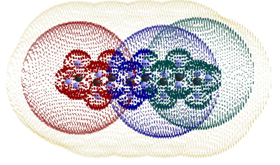
FIG. 3. A two level adaptive grid for an alkane: the high resolution grid points are shown with bold points while the low resolution grid points are shown with smaller points. Also visible are three localization regions (red, blue and green) with radii of 3.7 Å centered on different atoms in which certain support functions will reside. The coarse grid points shown in yellow do not belong to any of the three localization regions.
