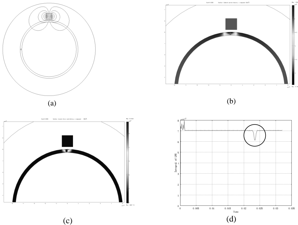
Fig 4. A Numerical model with moving meshes is built to investigate the main feathers of LFPA. The particle size is 50 \mu\text{m} , and the diameter of the wire is 1mm, and consequently the order of the force can be of the order of 10^{-7} [N].
