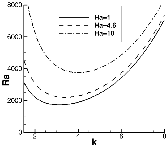
Fig. 2: Marginal stability curves for different Hartmann numbers. The minimum of each curve gives the critical values Ra_{crit} and k_{crit} .
