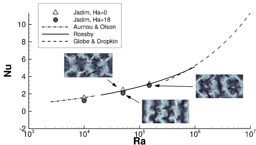
Fig. 6: Nusselt number as a function of the Rayleigh number for Ha=0 and Ha=18 .
