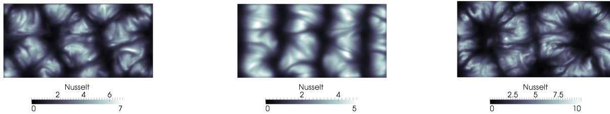
Fig. 5: Instantaneous local Nusselt number at the top walls for (from left to right): Ra and Ha were (from left to right): (i) Ra=5 \cdot 10^4 , Ha=0 , (ii) Ra=5 \cdot 10^4 , Ha=18 (iii) Ra=1.5 \cdot 10^5 , Ha=18 .
