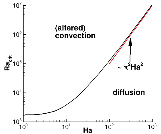
Fig. 3: Critical values of the Rayleigh number Ra_{crit} as a function of the Hartmann number.
