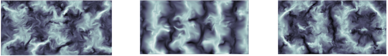
Fig. 4: Instantaneous snapshots of vertical velocity in the mid-plane z = e/2 , normalised by its maximal value (white is positive and black is negative). The values of Ra and Ha were (from left to right): (i) Ra = 5 \cdot 10^4 , Ha = 0 , (ii) Ra = 5 \cdot 10^4 , Ha = 18 (iii) Ra = 1.5 \cdot 10^5 , Ha = 18 .
