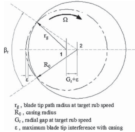
Fig. 2 Rub geometry
