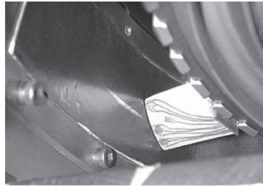
Fig. 12 Blade and casing after very light rub
