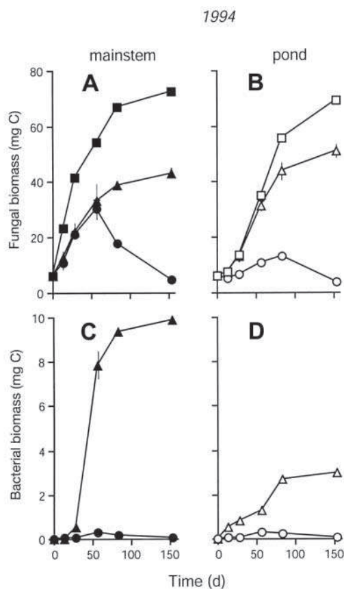
Fig. 4. Comparison of cumulative microbial production with actually observed biomass on decomposing leaves in the mainstem (A,C) and a floodplain pond (B,D) of the Garonne River system in 1994–95. ( \blacktriangle , \triangle ) Cumulative production values derived from instantaneous production rates ( [^{14}\text{C}] acetate (fungi) and [^3\text{H}] thymidine (bacteria) incorporation); ( \blacksquare , \square ) cumulative production values that include the separately determined conidial production; ( \bullet , \circ ) actually observed biomass. All values refer to 1 g of litter ash-free dry mass present before leaves were submerged. Bars denote \pm 1 SE ( n = 4 )
