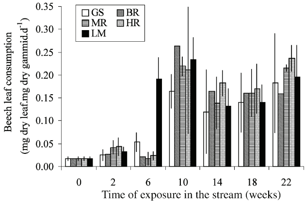
Fig. 2. Mean consumption of beech leaves conditioned in five headwater streams (GS, BR, MR, HR, LM), by G. fossarum . All values are means of 3 replicates \pm 1SD. * Means significant differences between streams (ANOVA, P<0.05 ).
