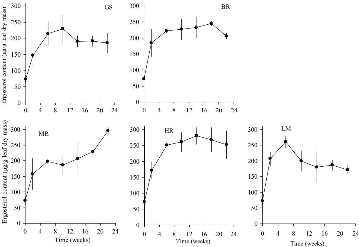
Fig. 1. Dynamics of ergosterol concentrations of aquatic fungi associated with decomposing beech leaves in five headwater streams. All values are means of 3 replicate leaf bags. Vertical bars represent \pm 1SD.
