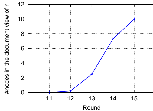
FIGURE 7 – System behaviour when a new document is added to node n
