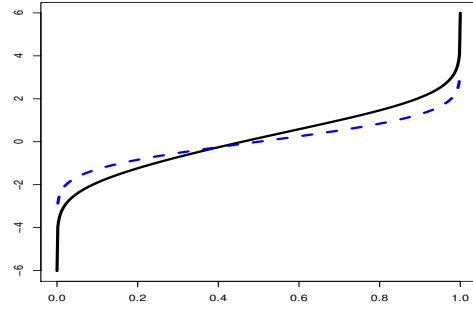
(c) Euclidean mean density \bar{f}_n (d) Quantile function of the arithmetical mean measure \bar{\nu}_n with density \bar{f}_n
