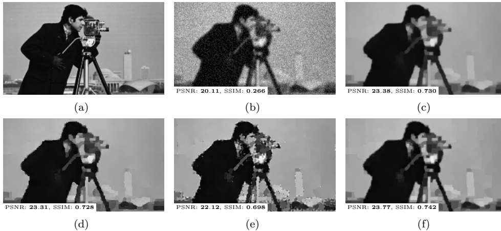
FIG. 14. (a) Original x_0 . (b) Blurred and noisy y = \Phi x_0 + w . (c) Original aniso-TV \hat{x}(y) with \lambda = 0.7 . Enhanced results by (d) iterative hard-thresholding, (e) post re-fitting with support identification, and (f) our proposed covariant re-fitting.
