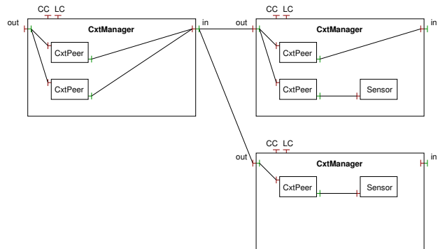
Fig. 6. Fractal-based component system modeling
