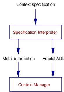
Fig. 4. Context specification processing
