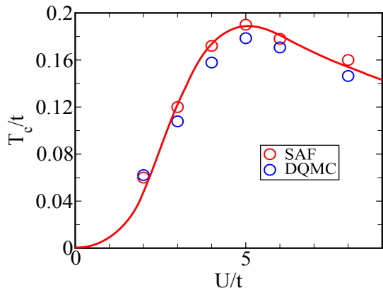
FIG. 5. Comparison of superfluid T_c obtained within our static auxiliary field (SAF) scheme, with DQMC (Ref. 15 of main text). The results are for a flat system with density n = 0.7 and lattice size 10 \times 10 .
