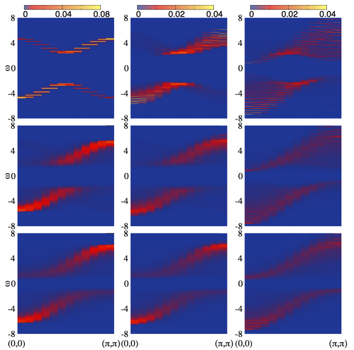
FIG. 4. Colour online: The spectral function A(\mathbf{k}, \omega) for a ‘diagonal scan’ from \mathbf{k} = \{0, 0\} \rightarrow \{\pi, \pi\} . Along the row, V_c varies from 0.1t, t, 3t (left to right). Down the column T varies from 0, 0.08t, 0.3t . The T_c of the unconfined system is \sim 0.14t , at V_c = 3t it is \sim 0.1t .
