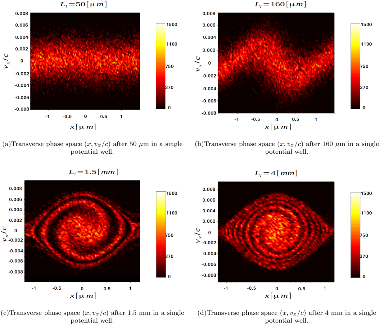
FIG. 5. Transverse phase space (x, v_x/c) for different interaction length. Simulation parameters: \gamma = 60 , \epsilon_N = 1 , \Sigma = 2 mrad, a_0 = 0.3 , L_R = 200 \mu\text{m} , \theta = 10^\circ , \lambda = 800 \text{ nm} . Note: free propagation a_0 = 0 .
