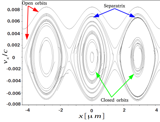
FIG. 3. Electron trajectories in the transverse phase space (x, v_x/c) . Simulation parameters: \epsilon_N = 1 mm mrad, \Sigma = 2 mrad, a_0 = 0.3 , L_R = 200 \mu\text{m} , \theta = 10^\circ , \lambda = 800 nm.
