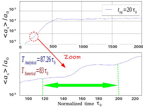
FIG. 11. Amplification of the scattered field in time. Simulation parameters: a_0 = 0.1 ; \lambda = 1 \mu m ; \theta = 10^\circ ; a_{seed} = 10^{-6} ; \Sigma = 3 \text{ mrad} ; \gamma = 10 ; \beta_\perp = 0.1 ; \delta\gamma/\gamma = 10^{-4} ; t_{inj} = 20 \tau_0 . Normalized electron density is n_e = 8 \cdot 10^{-5} . Macro-particles number is 2 \cdot 10^6 .
