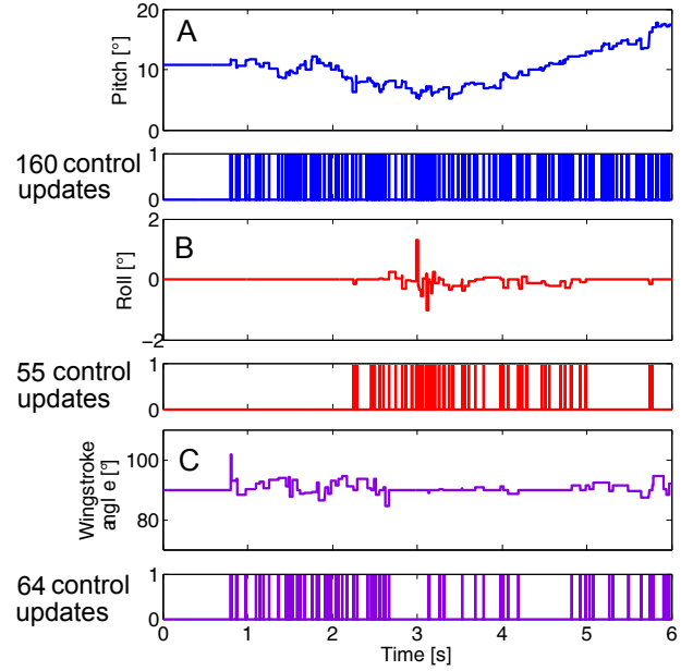
Fig. 3. Simulated control signals and control updates during a 3D trajectory starting at the initial coordinates x_0 = 0.1\text{m} ; y_0 = 0.5\text{m} ; z_0 = 0.3\text{m}
